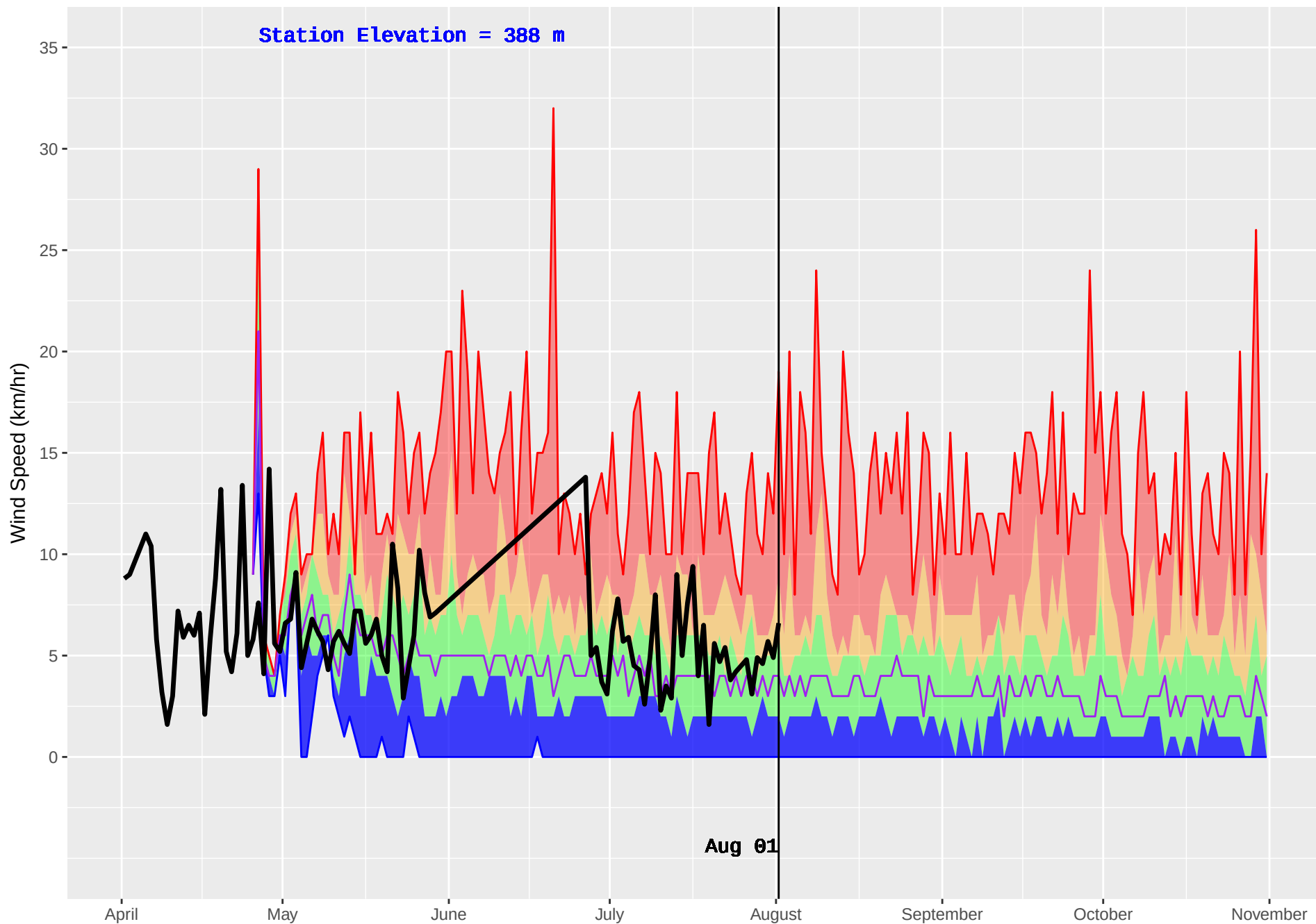
BELL-IRVING (432) : Historical (1986–2016) and Current (2018) Daily Wind Speed
